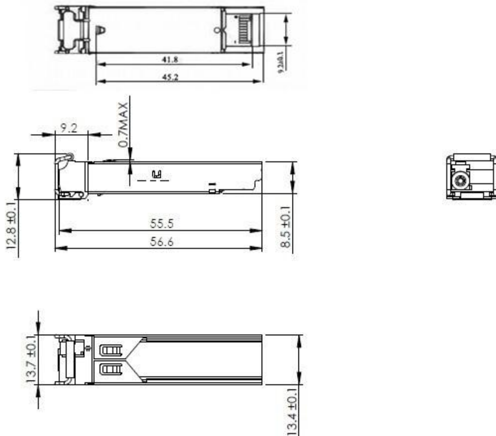
Mechanical Drawing
