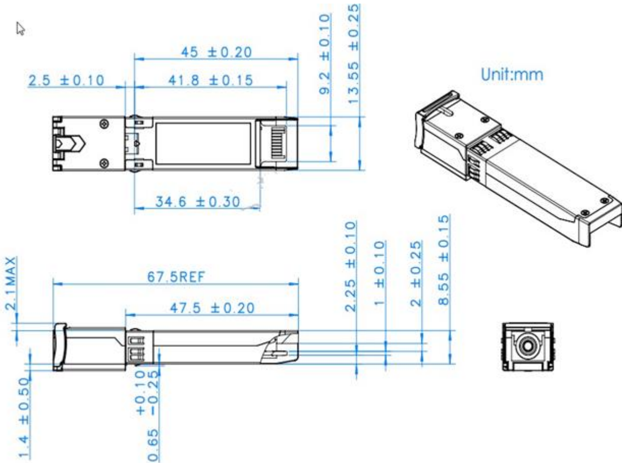
Figure 8 Package Outline
